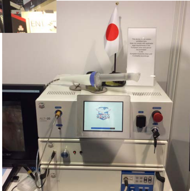
Asuka Laser Thermotherapy System at AMED Booth
